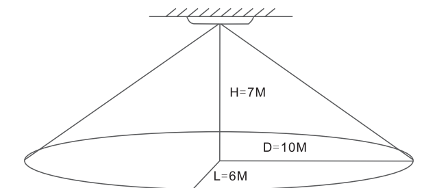
Microwave Detection
